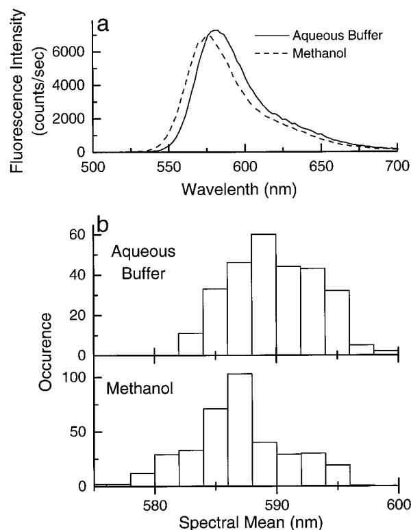
FIGURE 6 The effect of methanol on the fluorescence spectrum. (a) Ensemble fluorescence spectra of TMR-S1. The solid curve is a spectrum obtained in an aqueous buffer solution and the dashed curve in methanol. (b) Single molecule measurement of TMR-S1. Single molecule spectrum was measured and the spectral mean was calculated for each spectrum. The data of the spectral mean in aqueous buffer solution (top) and in methanol (bottom) are summarized in the histograms.
