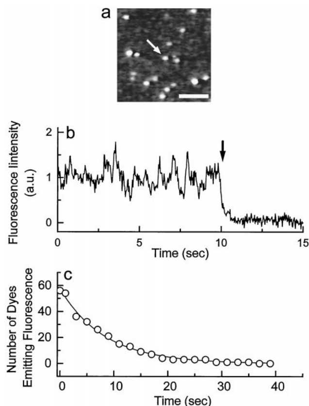
FIGURE 2 Fluorescence images of single TMR-S1 molecules in aqueous solution. (a) Fluorescence images. Single spots correspond to single TMR-S1 molecules (see text for details). The specimen was illuminated by an argon laser at 514.5 nm with the excitation power of 14 mW at the specimen plane. For emission, a bandpass filter of transmission wavelengths between 555 and 585 nm was used. The images were integrated over 16 video frames or 0.53 sec. Bar, 5 \mu\text{m} . (b) The time course of the fluorescence intensity from a single spot pointed by the arrow in (a). The laser power was 14 mW. The fluorescence dropped to baseline due to photobleaching at the time indicated by an arrow. (c) The exposure time until photobleaching was measured for individual molecules, and the data were summarized by counting the number of molecules remaining fluorescent and plotting it as a function of time. The decay is fitted to a single exponential function with a rate constant of 0.12 \text{ sec}^{-1} (solid curve).
